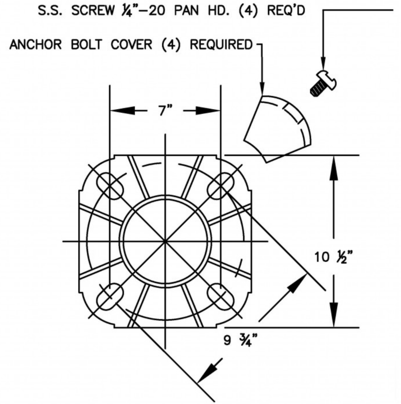
SHOEBASE PLAN CAST ALUM ALLOY A-356-T6
