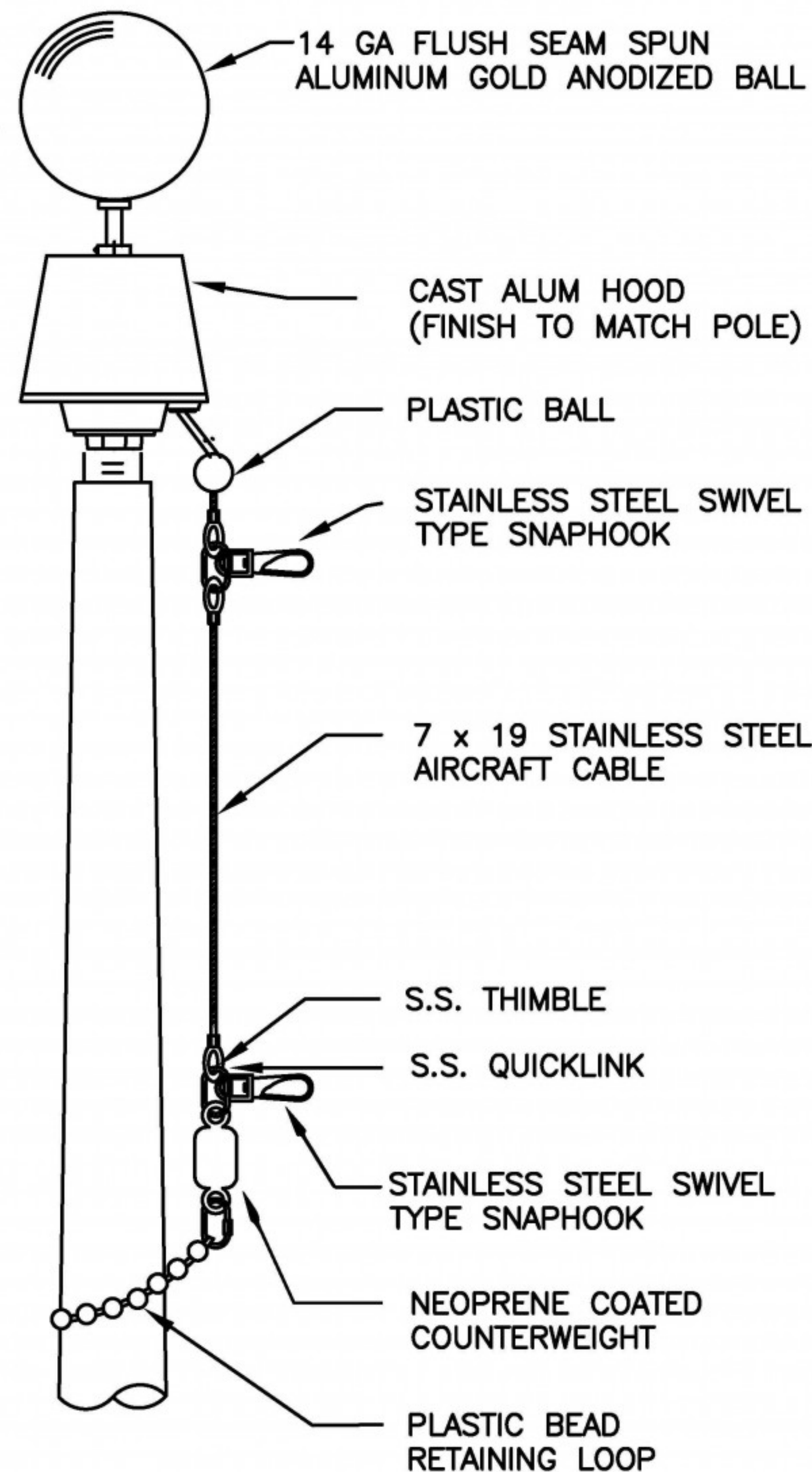
HOOD, TRUCK & RIGGING DETAILS
